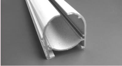
Contempra aluminum head rail with Velcro™ (white) for Toxa mechanism.
